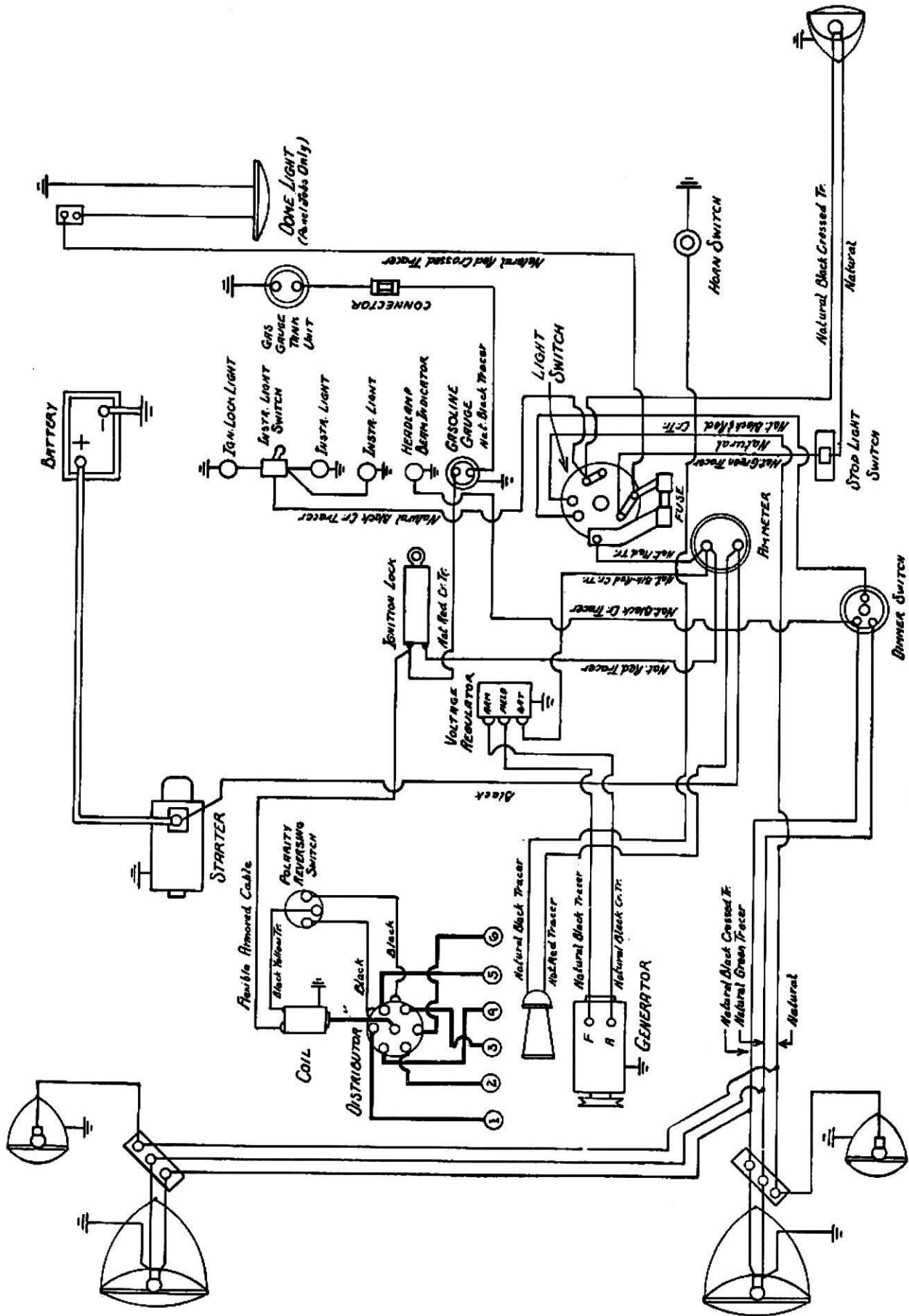
Fig. 66—Truck Wiring Diagram
