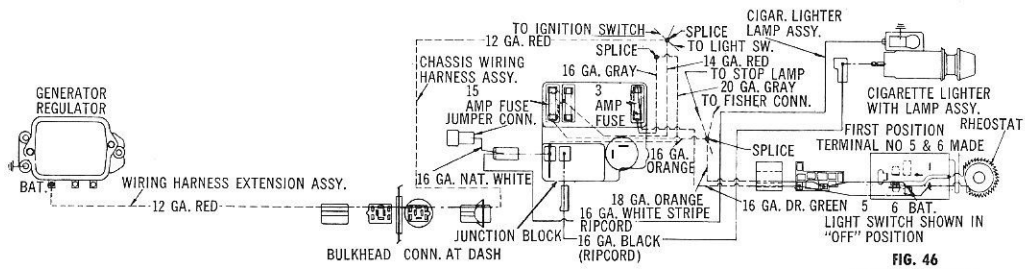
FIG. 46 CIGARETTE LIGHTER CIRCUIT (EX. IMPALA)
