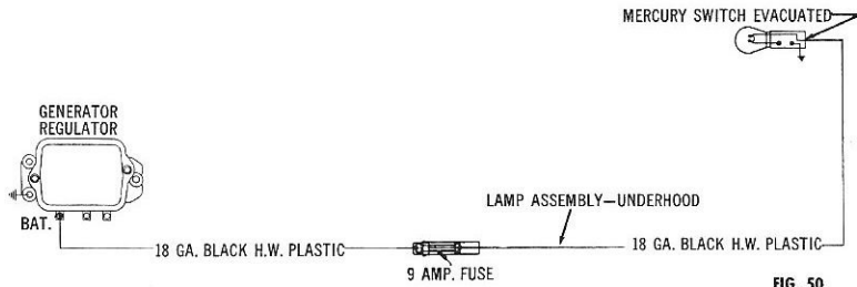
FIG. 50 UNDERHOOD LAMP CIRCUIT
