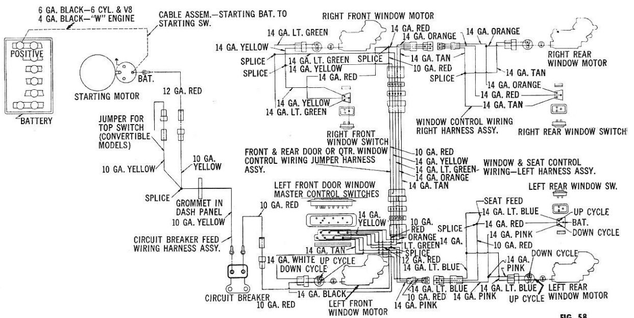
FIG. 58 POWER WINDOW CIRCUIT
