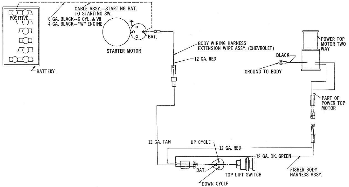
FIG. 57 POWER TOP (CONVERTIBLE) CIRCUIT
