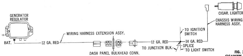
FIG. 36 CIGARETTE LIGHTER CIRCUIT
