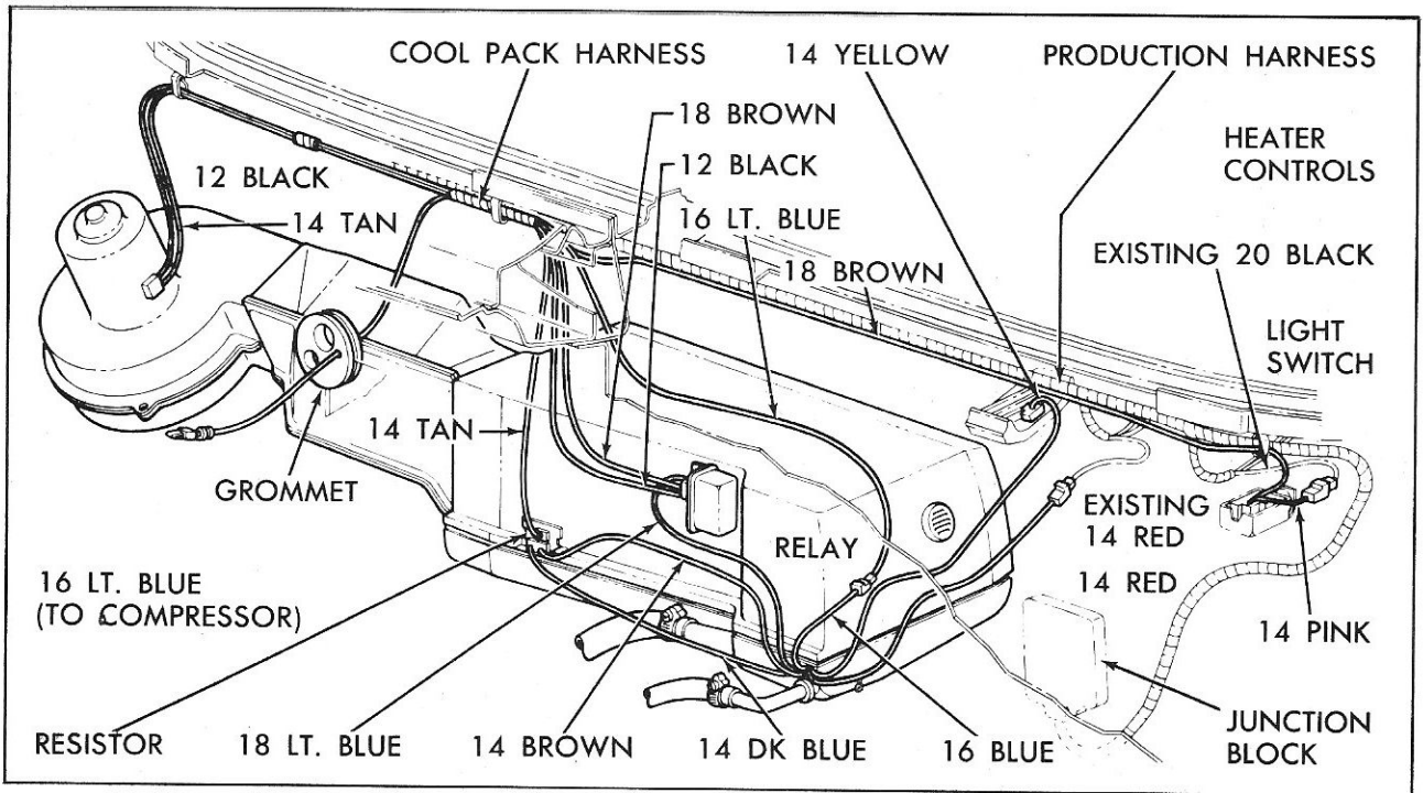
Fig. 35—Rear View of Evaporator—1960
