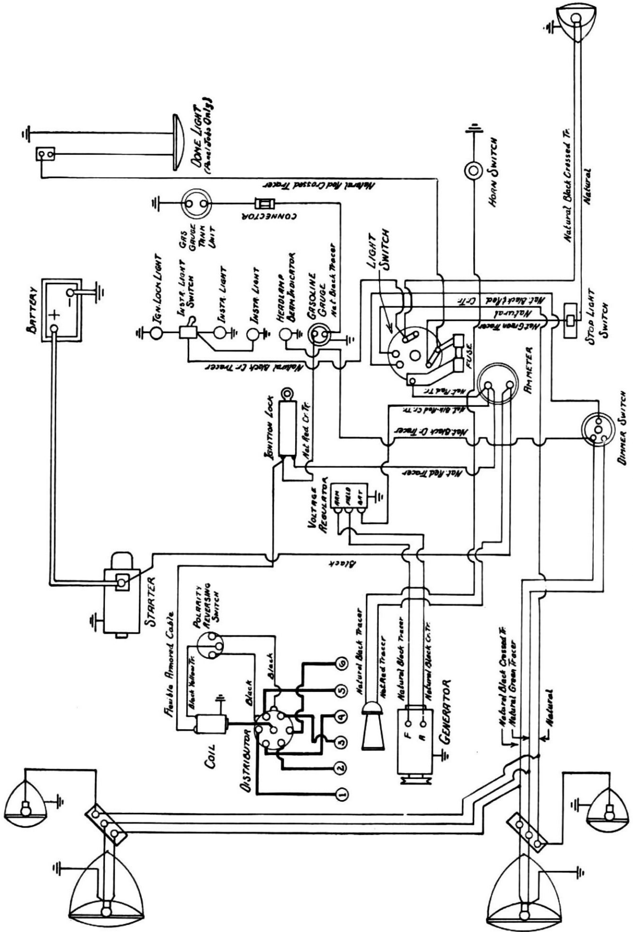
Fig. 60—Passenger Car Wiring Diagram 1941
