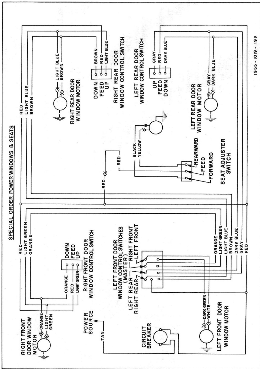
Fig. 98—Wiring Diagram Electric Windows and Seat
