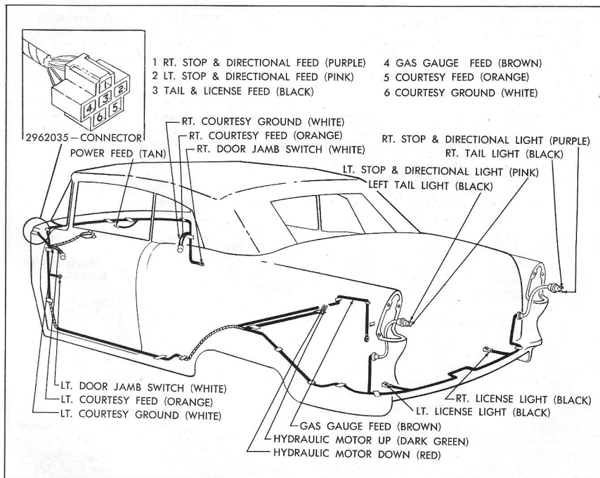
Fig. 121—Convertible Wiring Diagram
