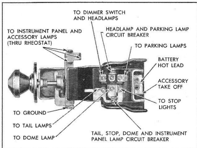
Fig. 3—Lighting Switch
