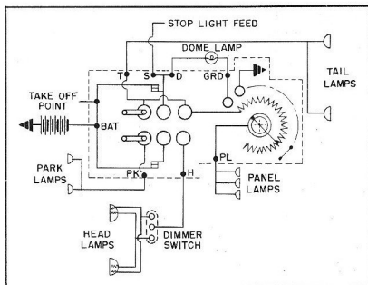
Fig. 4—Lighting Switch Circuit Diagram
