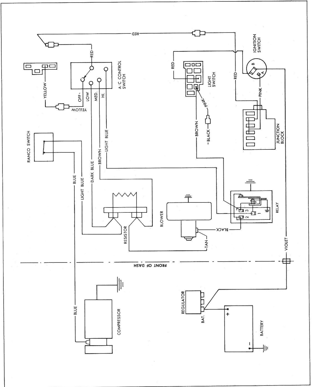
Fig. 37—Wiring Diagram, 1959 Cool Pack Air Conditioning System
