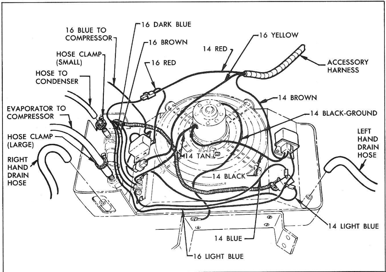
Fig. 34—Rear View of Evaporator—1959
