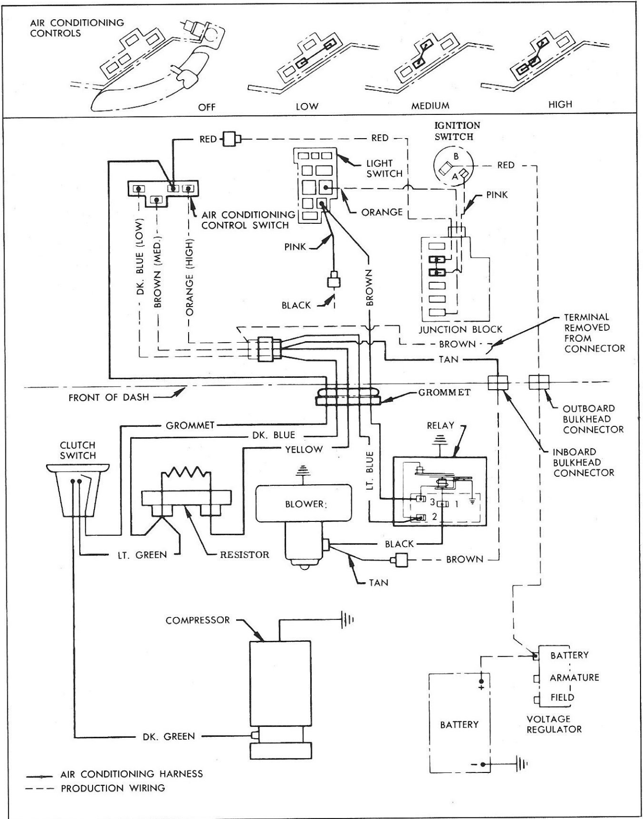
Fig. 14—Wiring Diagram, All-Weather Air Conditioning System
